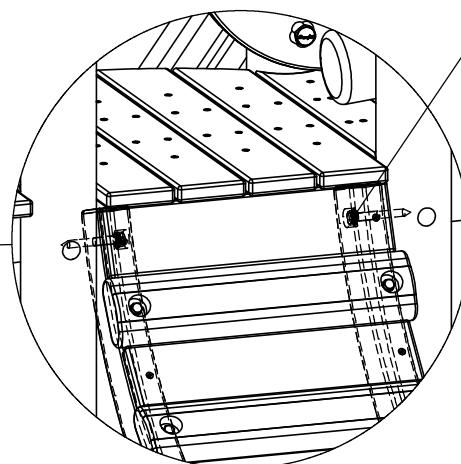
M10x80 2x
