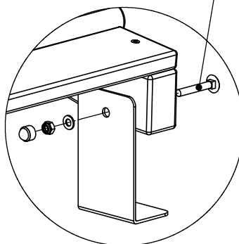
M8x55 2x
